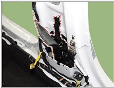
1) Front Seatbelt Pretensioner
